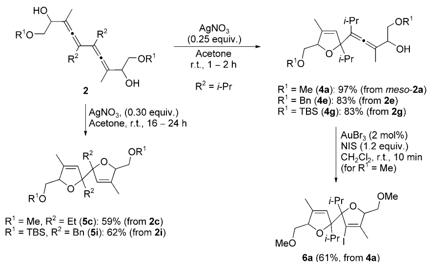
Scheme 4. Silver- and gold-catalyzed cycloisomerization of bis( \alpha -hydroxyallenes) 2 .
