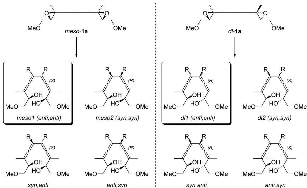
Scheme 3. Possible diastereomers of bis(α-hydroxyallenes).
