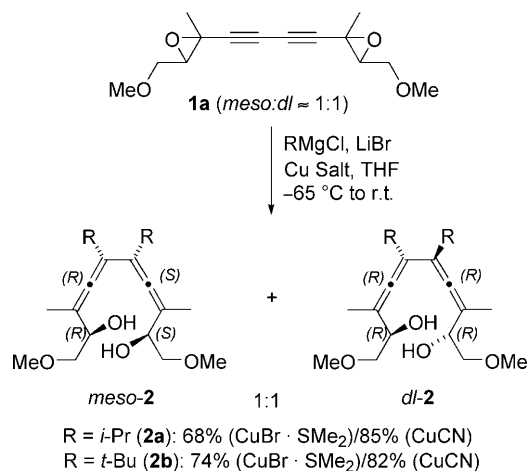
Scheme 2. Copper-mediated S N 2'-substitution of bisoxirane 1a to bisallenols 2a/b .
